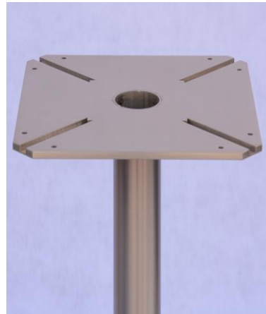
Top plate with custom cord grooves and hole in top plate.
